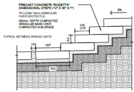
8 PRECAST CONCRETE STEPS SCALE 1:20
