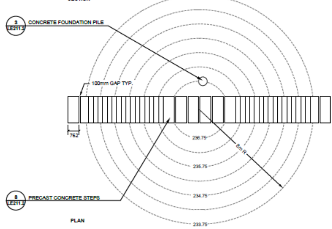
9 LARGE MOUND SCALE 1:100
